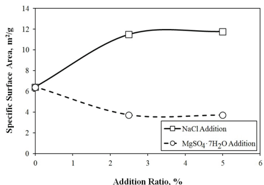
Figure 1. Variation of specific surface area with % addition
